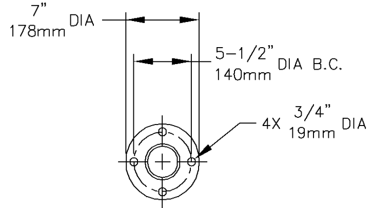
MOUNTING PATTERN
