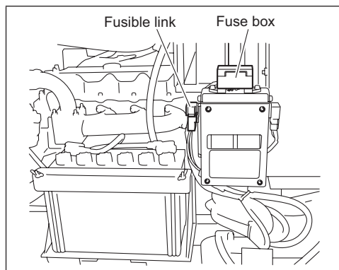
Fuse box
